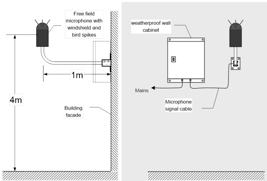
Figure 2: Typical long term EM2030 installation
